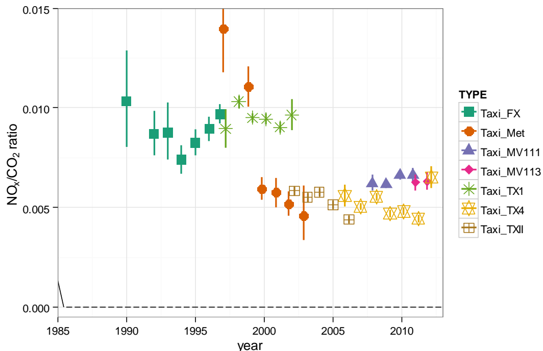
Figure 25 \text{NO}_x/\text{CO}_2 emissions from London taxis by year.
