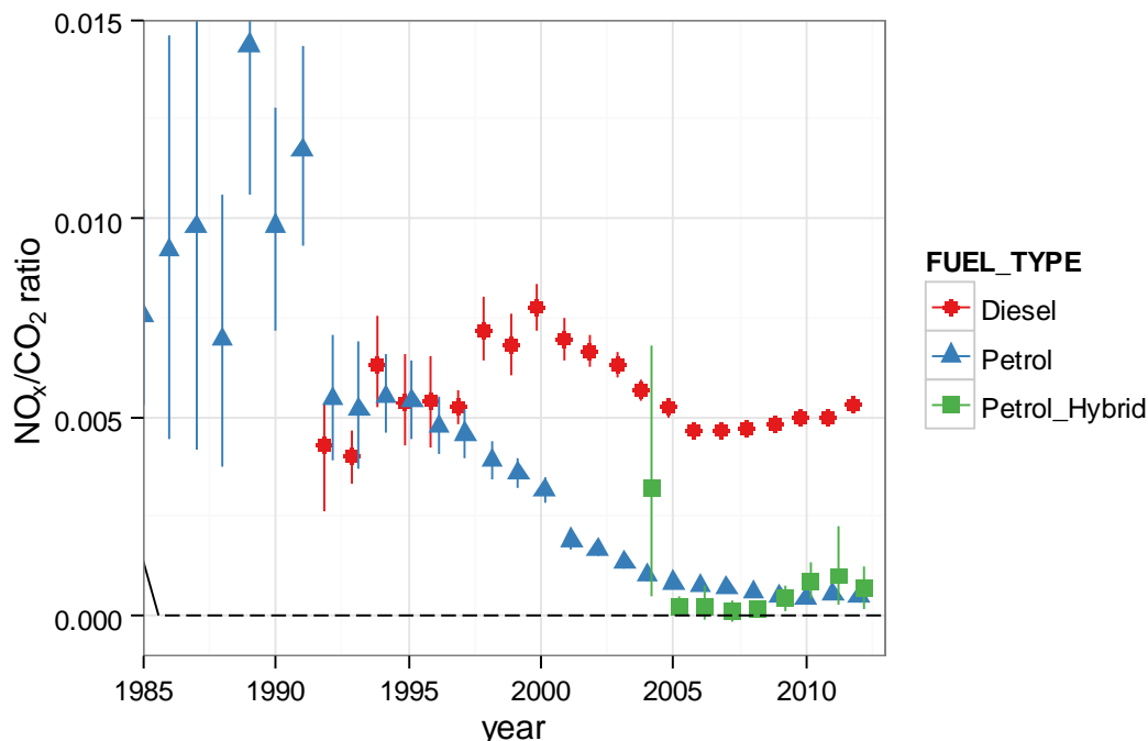
Figure 11 Trends in \text{NO}_x/\text{CO}_2 emission ratios for passenger cars by year of manufacture.
