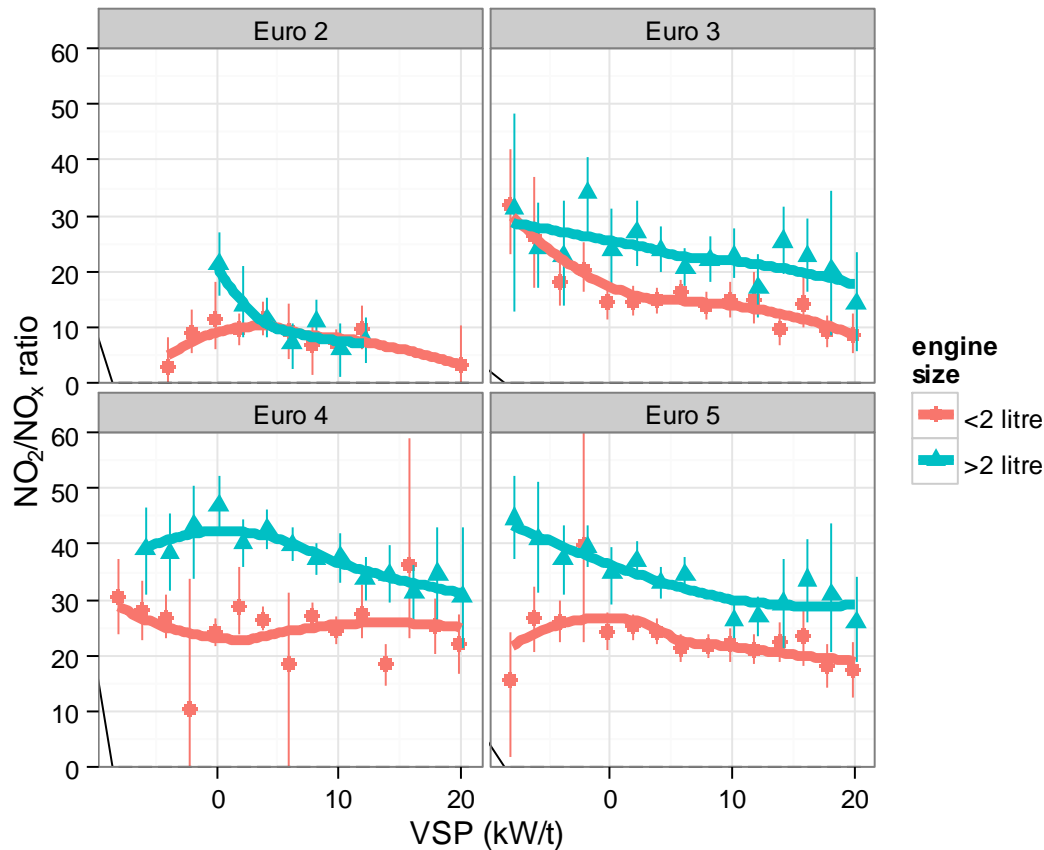
Figure 17 Relationship between vehicle specific power and emissions of NO 2 split by Euro class and engine size for diesel cars.
