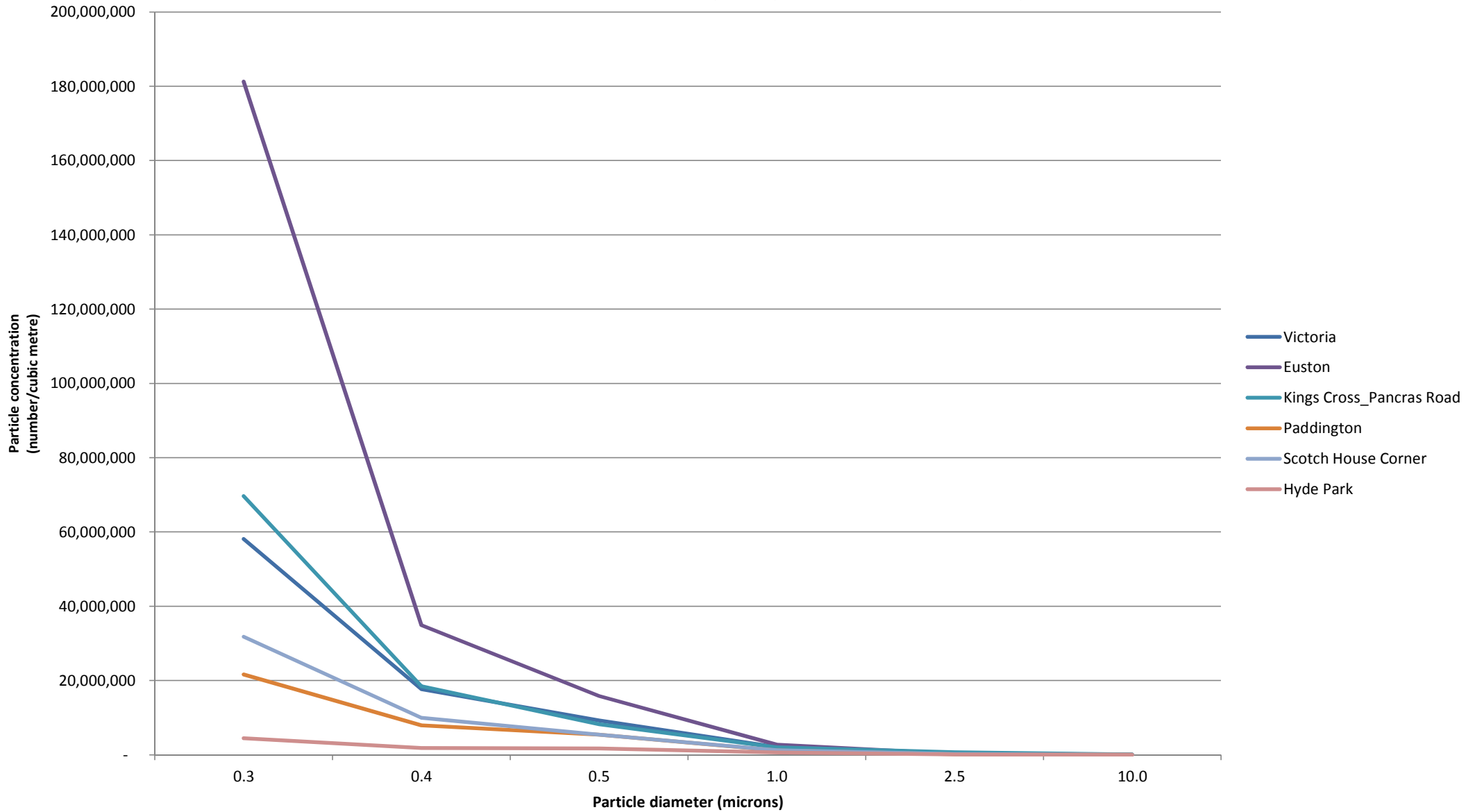
Particle concentration distribution Taxi ranks at four London stations on 26 January 2012 (plus Scotch House Corner and Hyde Park)
