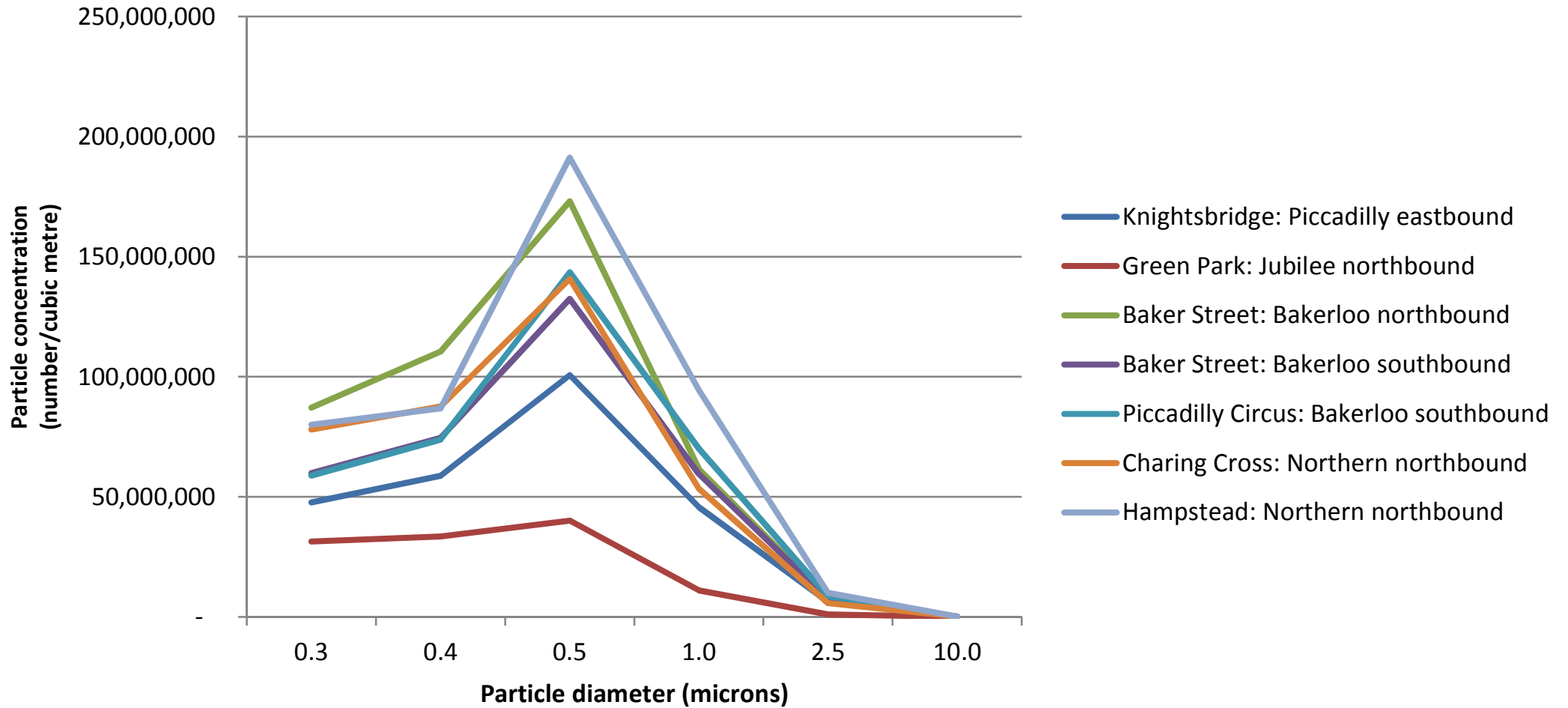
Particle concentration distribution London Underground platforms on 9 December 2011
