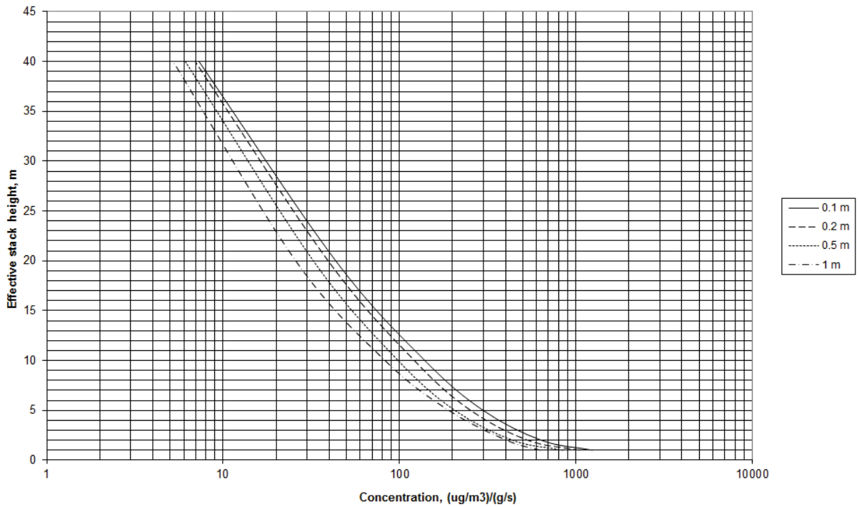
Figure A4.9: Maximum annual mean ground level concentration for 1 g/s emission rate-condensing boiler
