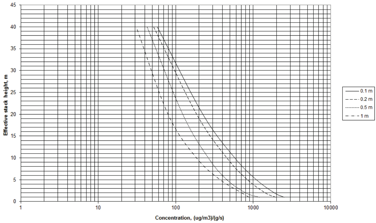
Figure A4.10: Maximum 99.8 h percentile 1 hour mean ground level concentration for 1 g/s emission rate-condensing boiler
