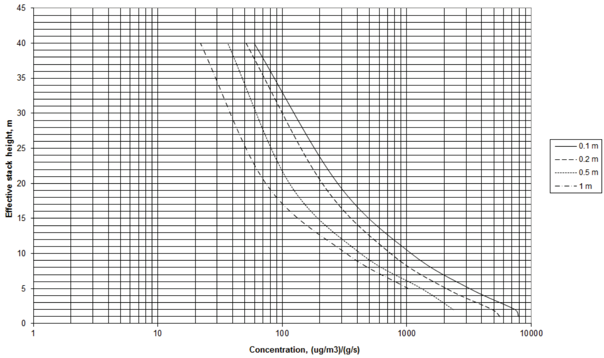
Figure A4.3: Maximum 99.8 th percentile 1 hour mean ground level concentration for 1 g/s emission rate-biomass boiler
