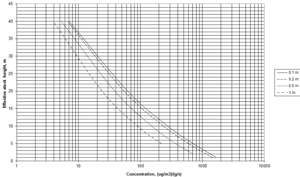
Figure A4.2: Maximum annual mean ground level concentration for 1 g/s emission rate-biomass boiler
