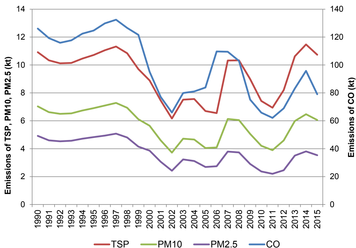
Figure 2-11 UK Emissions of CO, TSP, PM 10 and PM 2.5 from Iron & Steel Production (1990-2015)
