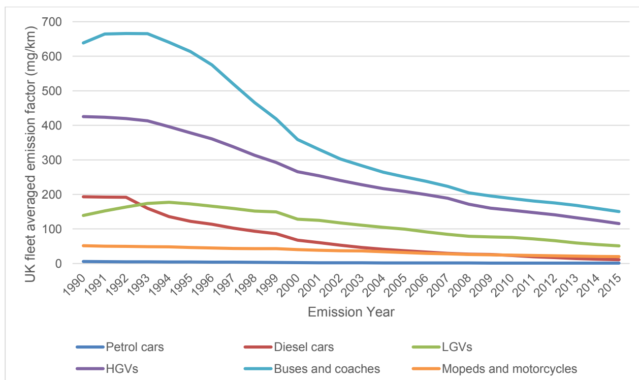
Figure 3-5 UK fleet averaged PM 10 hot exhaust emission factors for road transport
