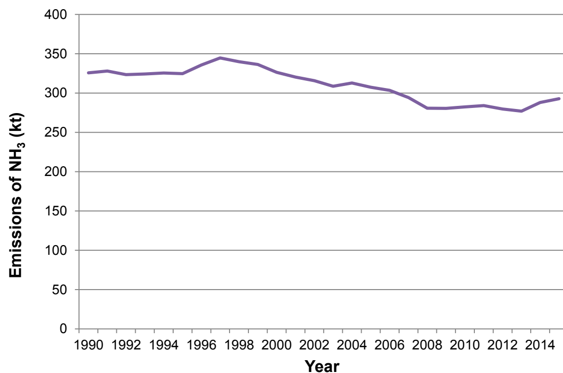
Figure 2-4 Total UK emissions of NH 3 for 1990 – 2015
