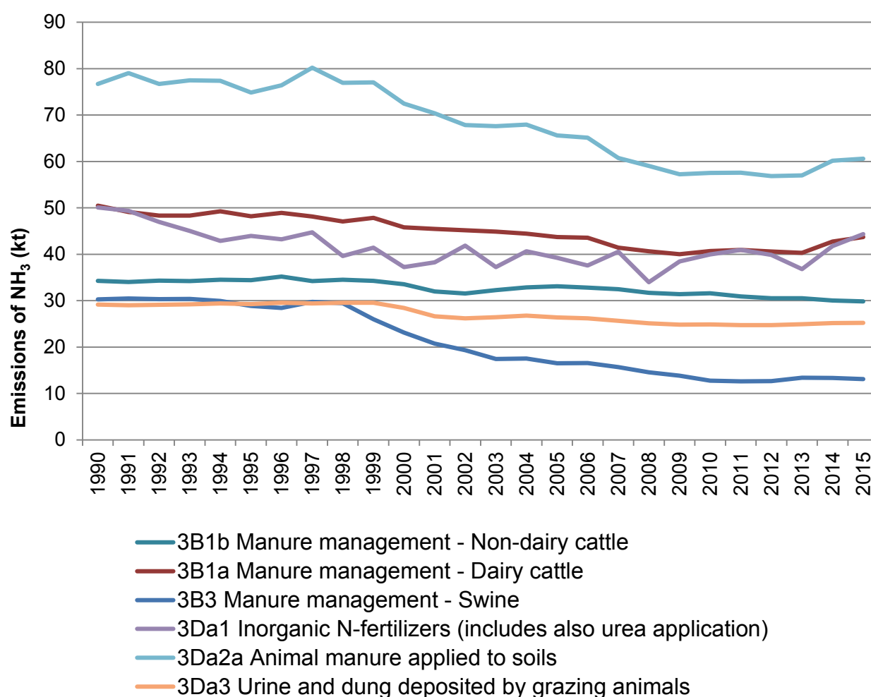
Figure 2-14 UK Emissions of NH 3 from Key Sources in Agriculture (1990-2015)
