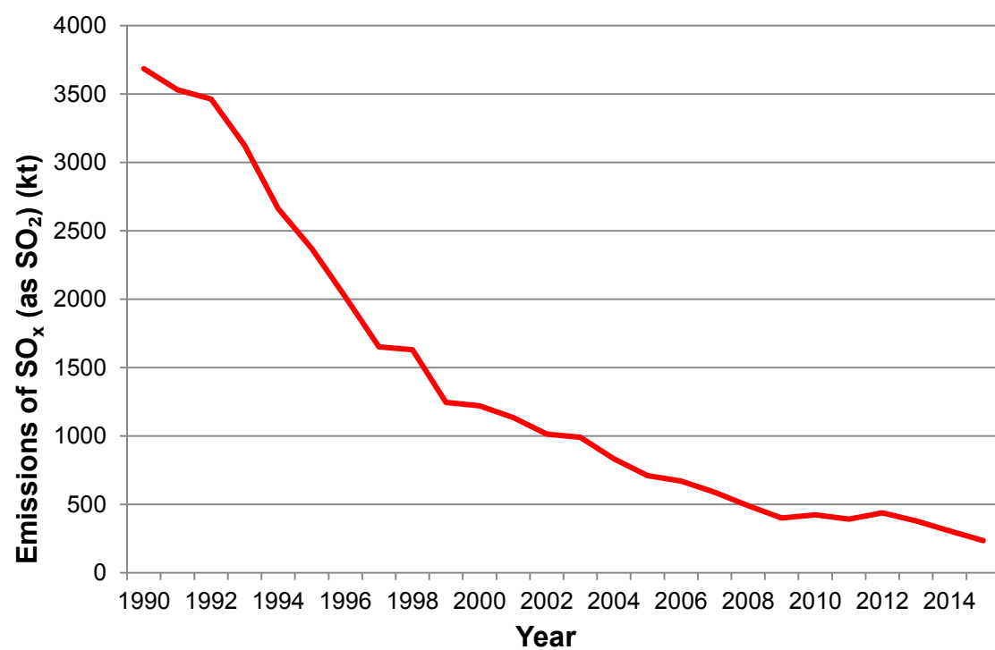
Figure 2-2 Total UK emissions of SO x (as SO 2 ) for 1990 – 2015
