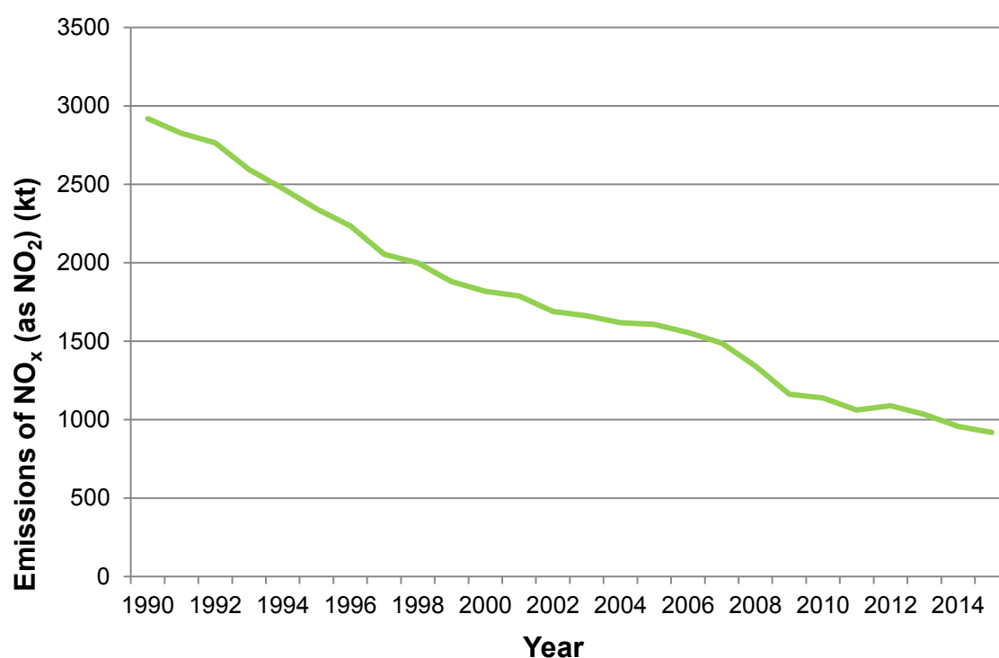
Figure 2-1 Total UK emissions of NO x (as NO 2 ) for 1990 – 2015
