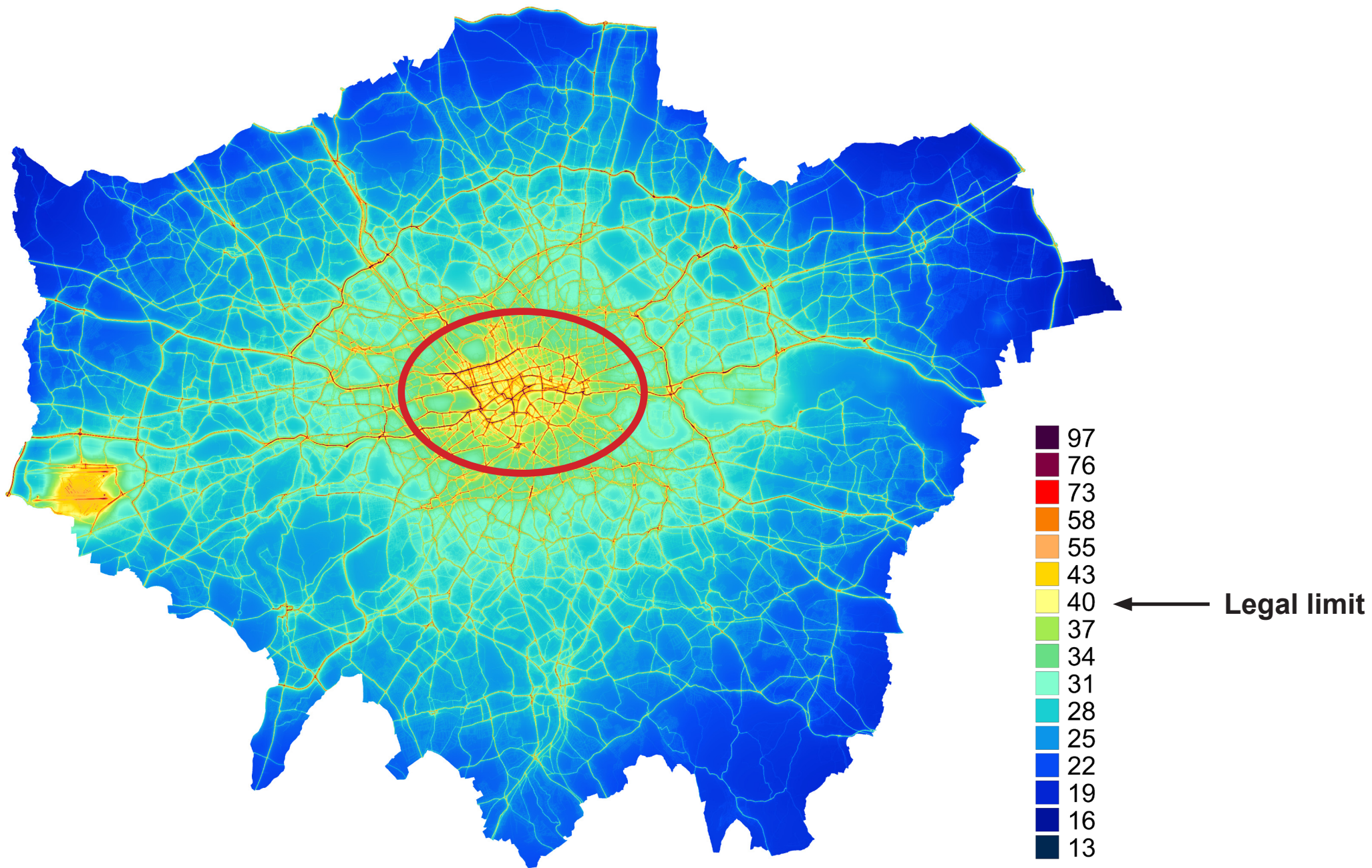
NO 2 annual mean concentrations in 2020 ( \mu\text{g}/\text{m}^3 )
