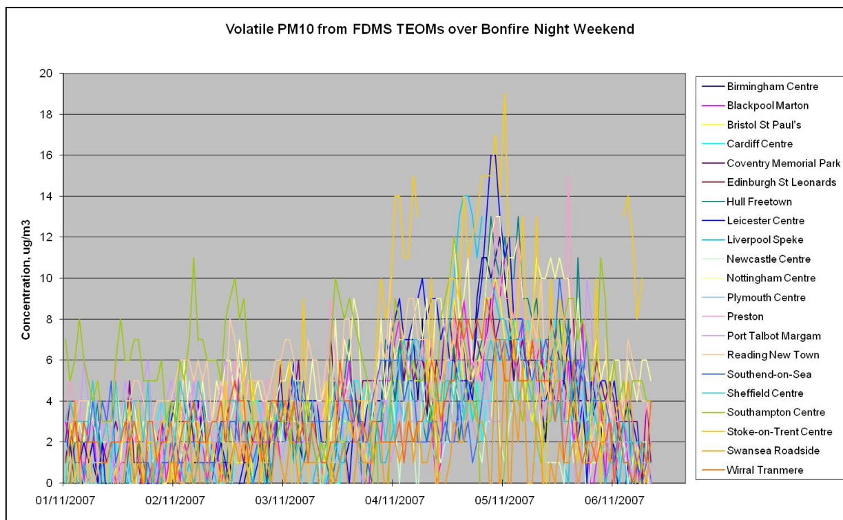
Figure 1.9 Selected PM 10 volatile concentrations from FDMS TEOM monitors
