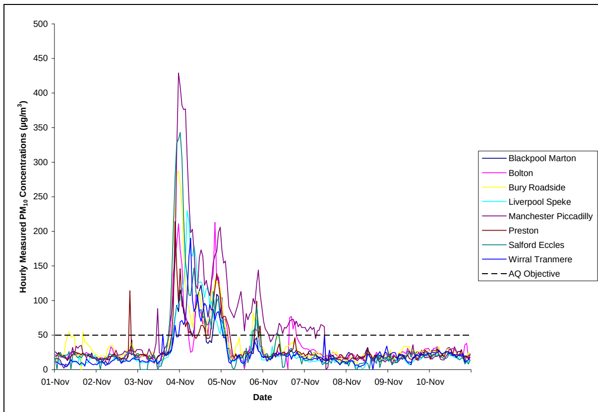
Figure 1.1 Hourly Measured PM 10 Concentration in the North West of England
