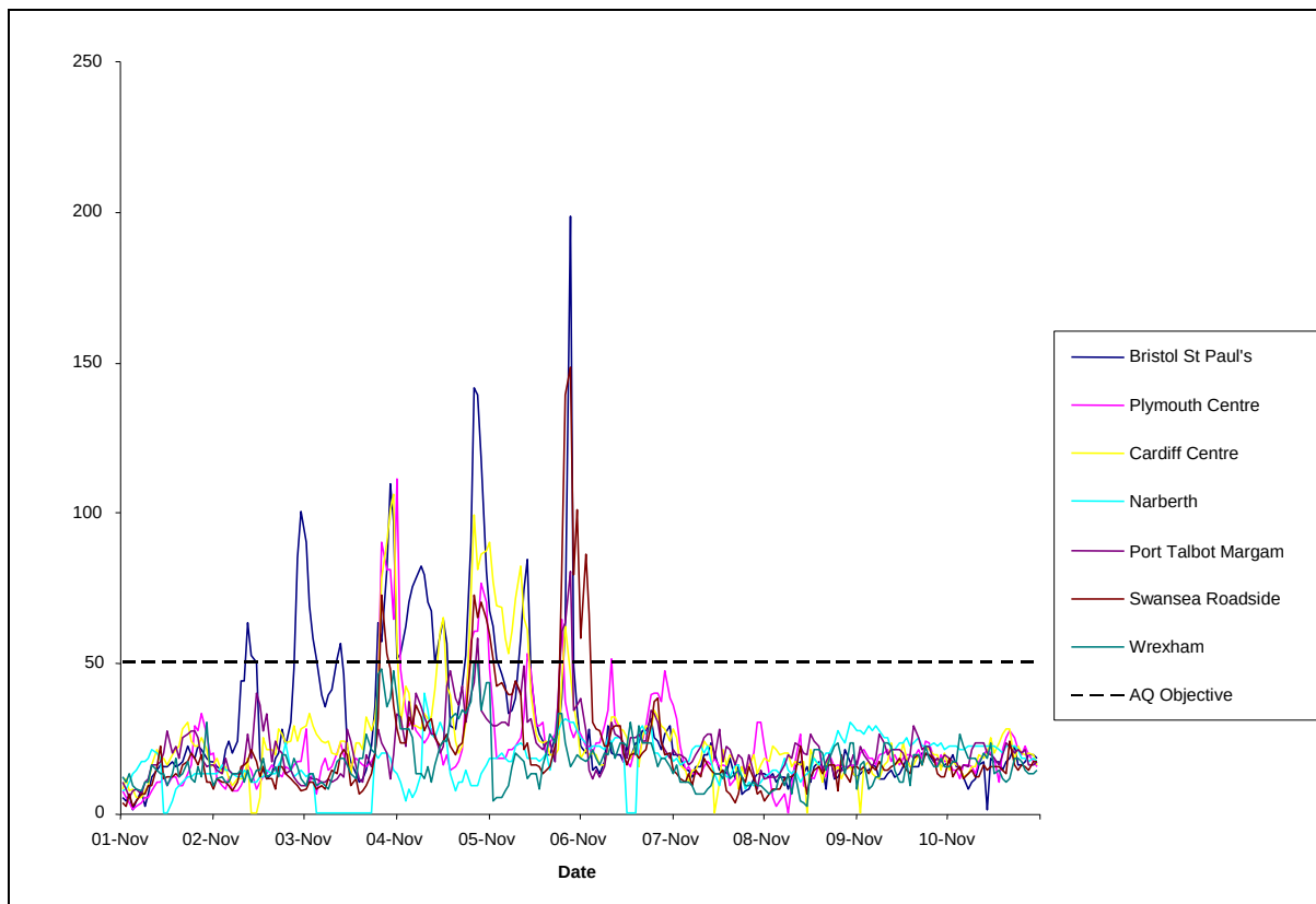
Figure 1.6 Hourly Measured PM 10 Concentration in the South West of England and Wales
