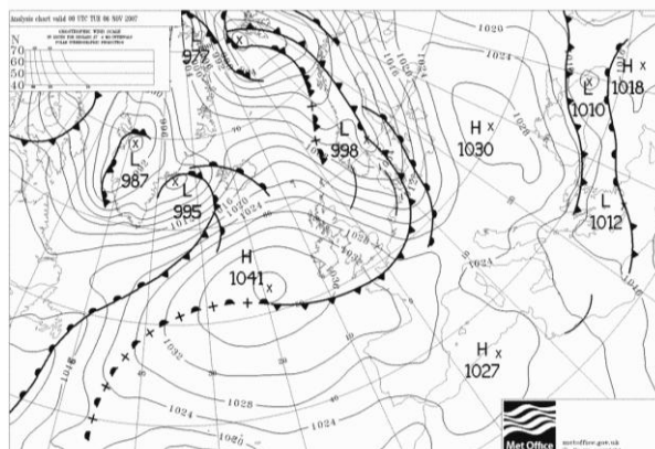
Figure 3.5 Met Office Surface Pressure Chart: 00 UTC Tuesday 6 th November
