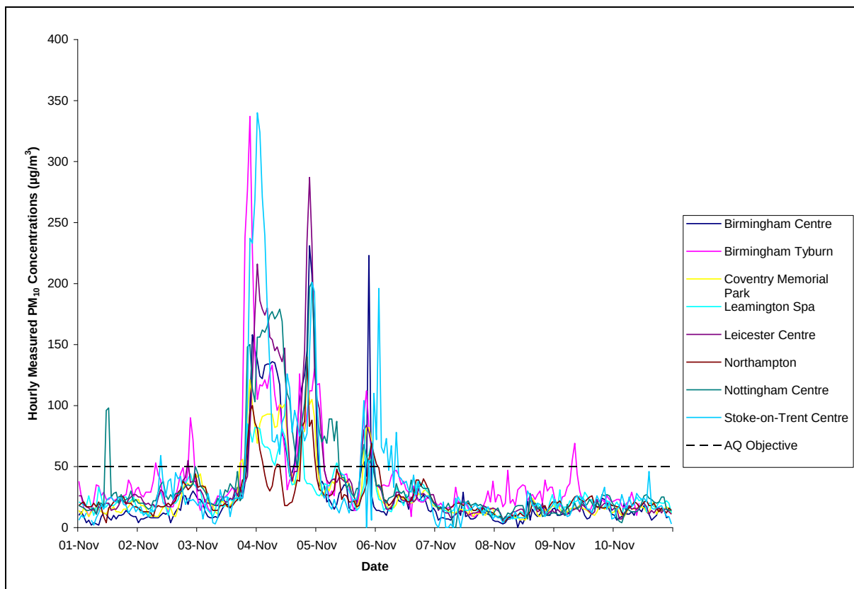
Figure 1.4 Hourly Measured PM 10 Concentration in the Midlands
