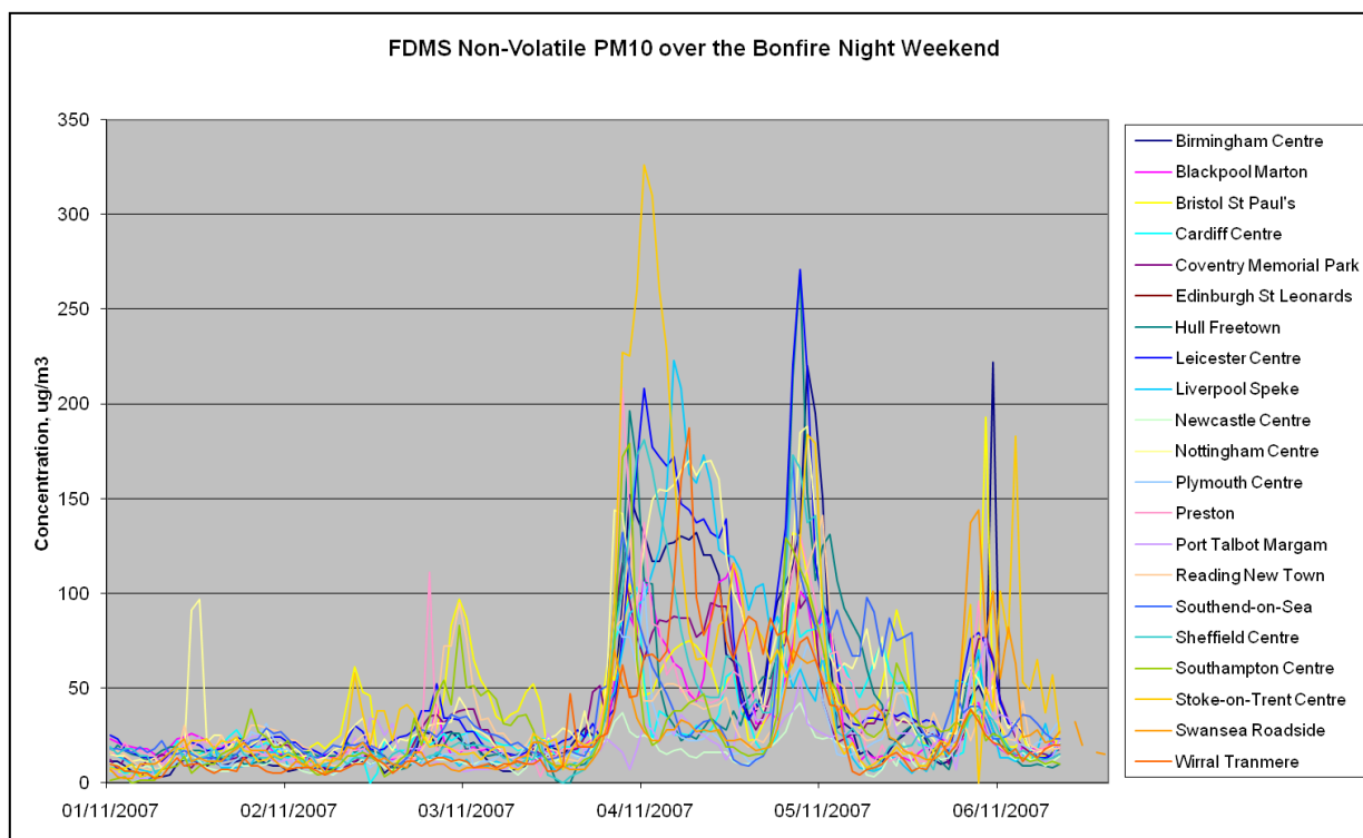
Figure 1.10 Selected PM 10 non-volatile concentrations from FDMS TEOM monitors
