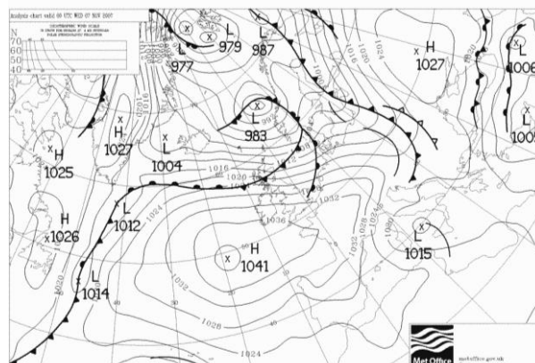
Figure 3.6 Met Office Surface Pressure Chart: 00 UTC Wednesday 7 th November
