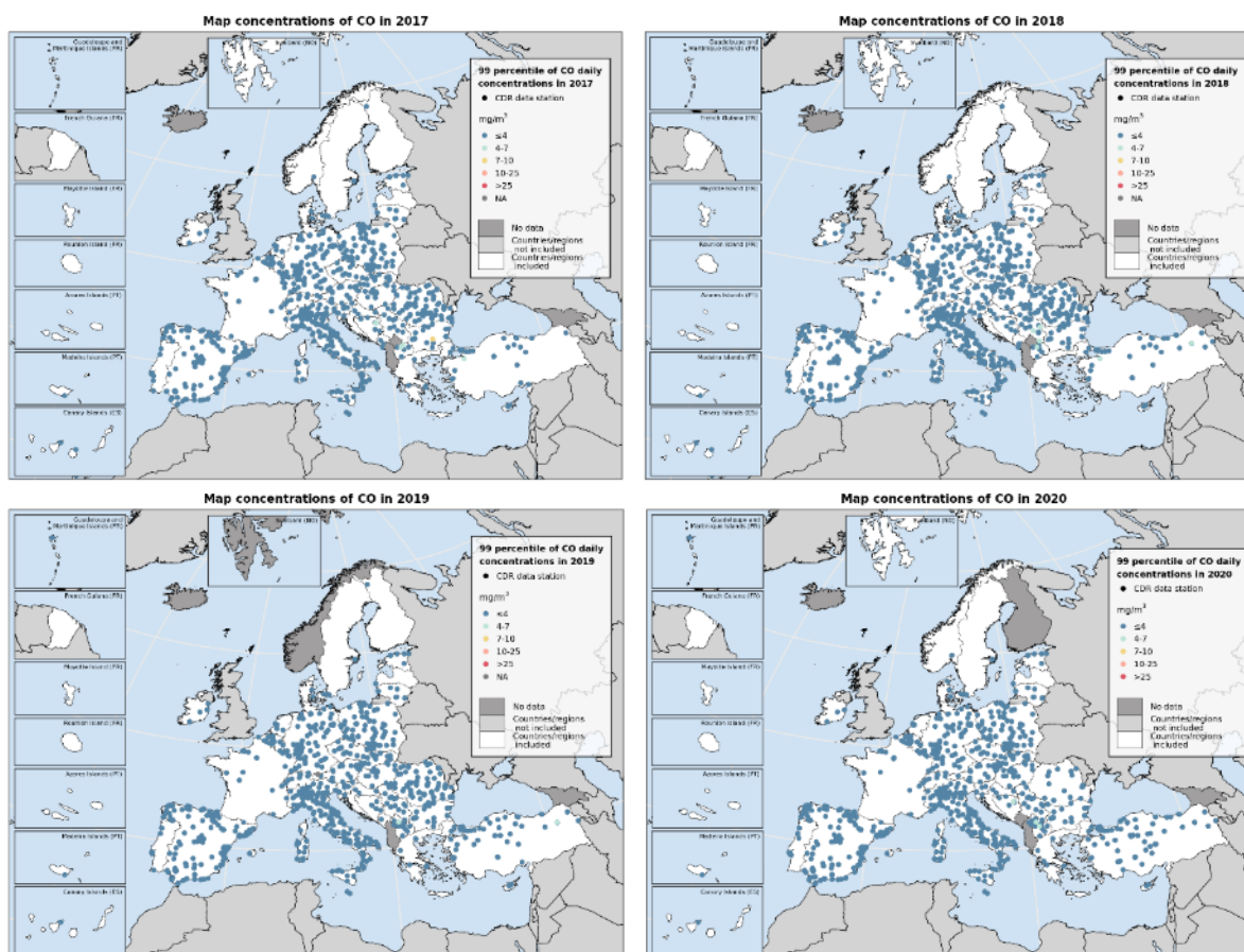
Figure A11.18 - CO daily mean concentrations for 2017 to 2020
