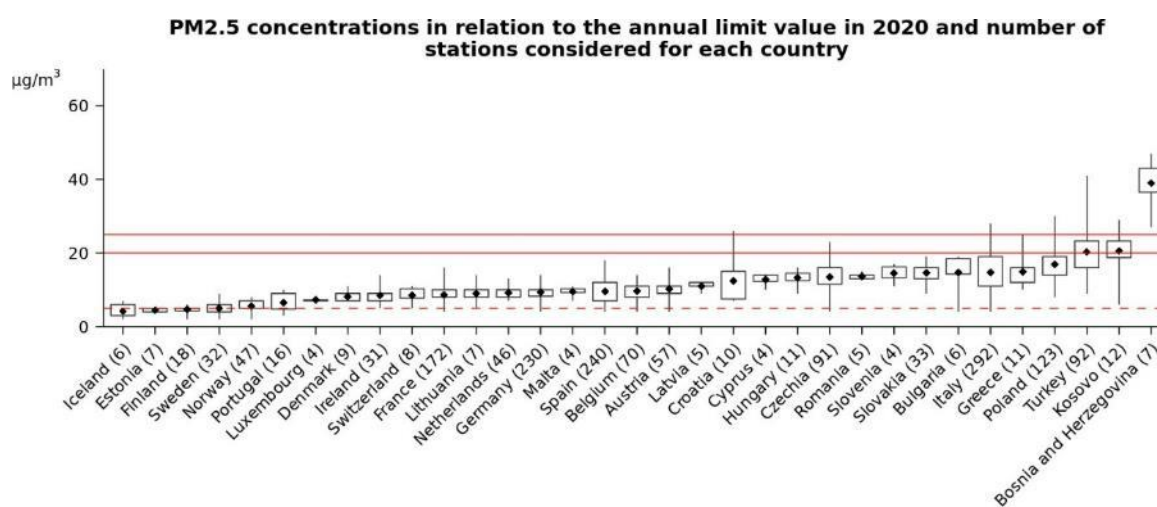
Figure A11.1 - PM 2.5 concentrations in relation to the annual limit value in 2020 by country. 179
