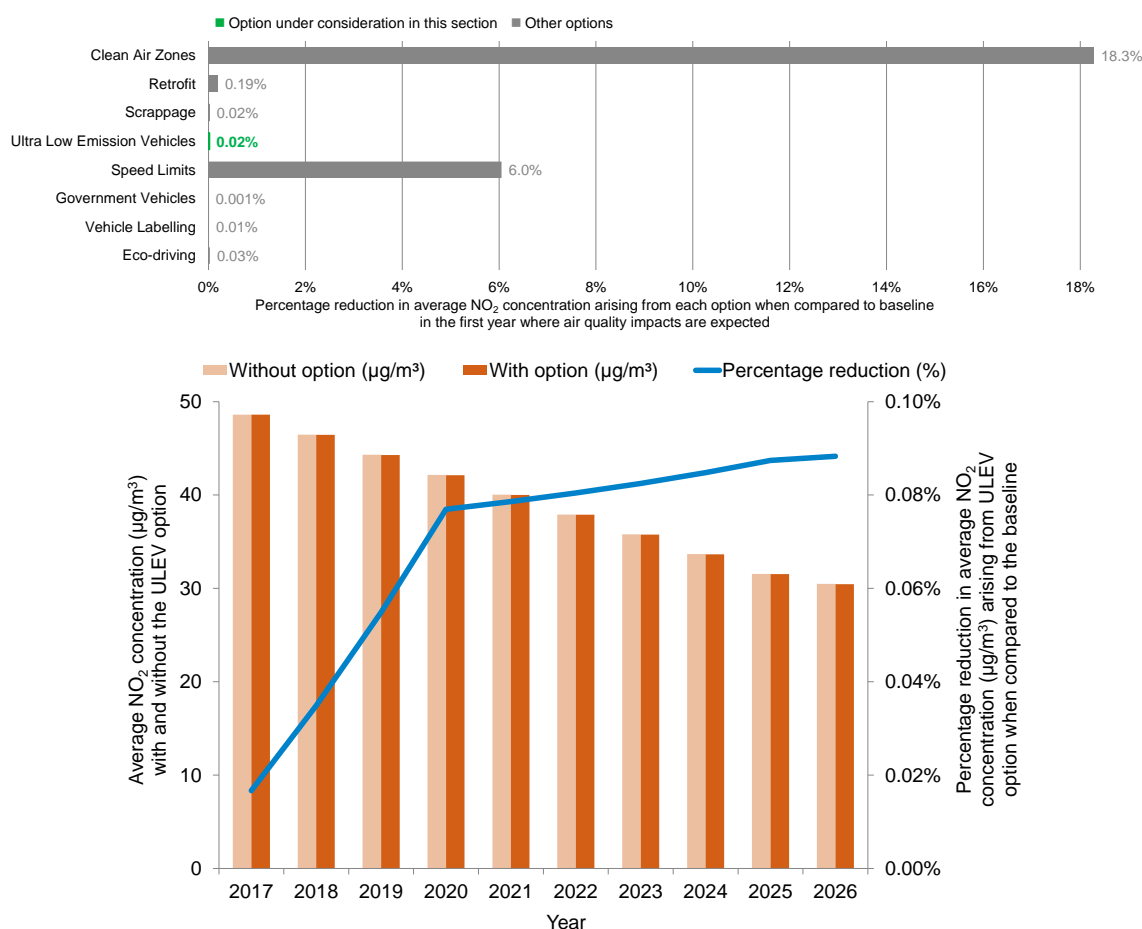
Figure 5.7: Reduction in average NO 2 concentrations following the implementation of the support for Ultra Low Emission Vehicles (ULEVs) option
