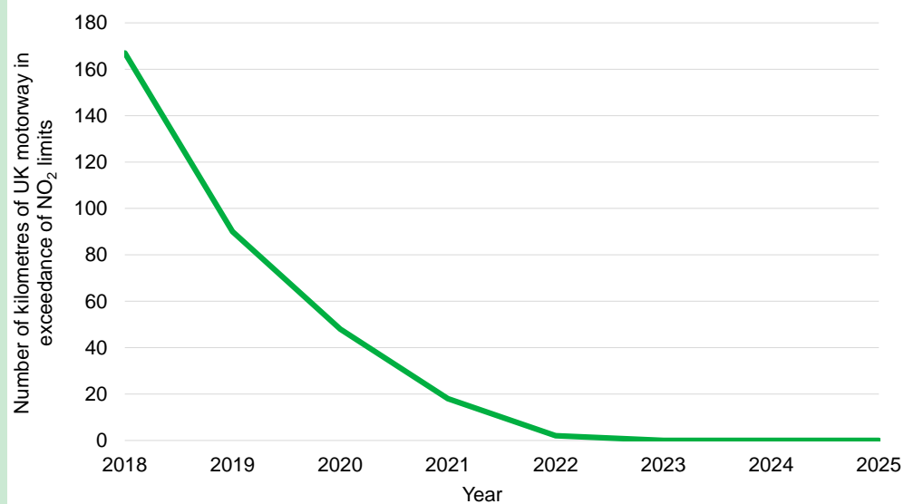
Figure 6.2: Projection profile for the number of kilometres of UK motorway in exceedance of \text{NO}_2 limits from 2018 to 2025
